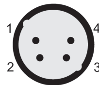
XLR-4M
